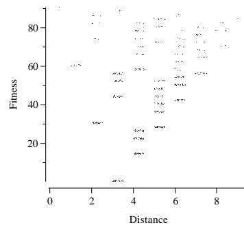
Figure 68. Three copies of Goldberg, Deb & Korb's fully deceptive 3-bit problem ( r = 0.32 ).
