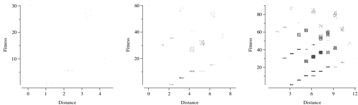
Figure 77. Whitley's F3. A Figure 78. Two copies of Whitley's F3 ( r = 0.37 ). Figure 79. Three copies of Whitley's F3 ( r = 0.37 ).
