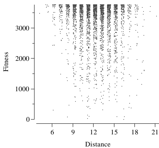
Figure 99. De Jong's F2 binary coded with 24 bits converted to a maximization problem ( r = -0.09 ).
