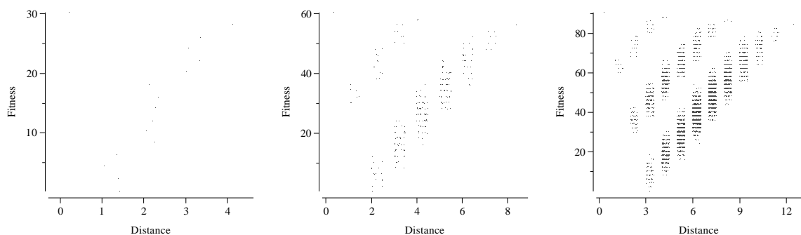
Figure 74. Whitley's F2. A Figure 75. Two copies of Whitley's F2 ( r = 0.51 ). Figure 76. Three copies of Whitley's F2 ( r = 0.51 ).
