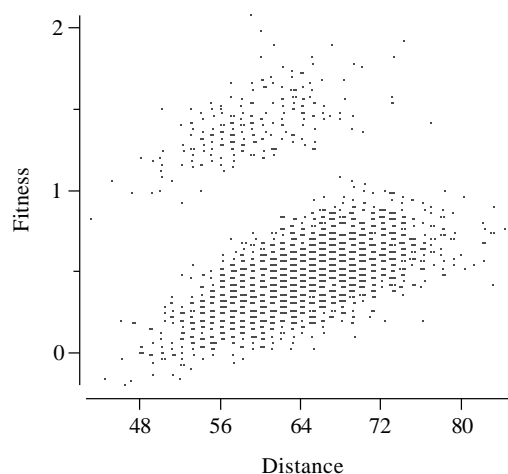
Figure 81. Holland's royal road on 128 bits ( b = 8 , k = 4 and g = 0 ), ( r = 0.27 , 4000 sampled points).
