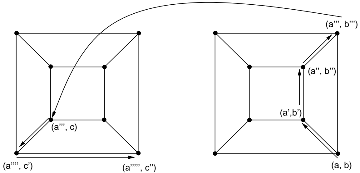
Figure 12. A fragment of a hillclimb under crossover. Three uphill steps are taken (using crossover) within the right hypercube, from (a, b) to (a''', b''') . At that point b''' is discarded and replaced with the randomly generated c . Two more steps are then taken on the left hypercube. The jump into the left hypercube is either the result of a limit on the number of steps in a hypercube (max-steps) or a limit on the number of attempts to find an improving crossover (max-attempts).
